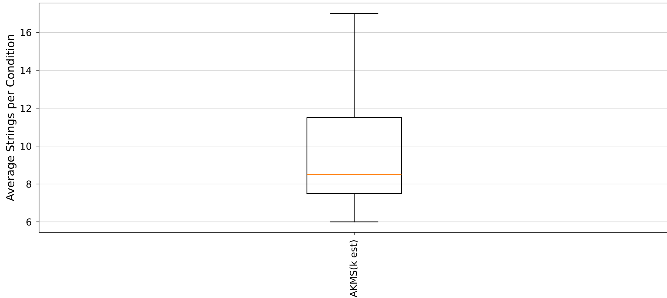
YARA Rules Average Strings per Condition Distribution (Cluster17_Size8 dataset)
